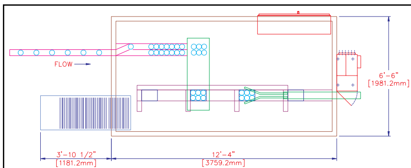
Standard Range Floorplan
